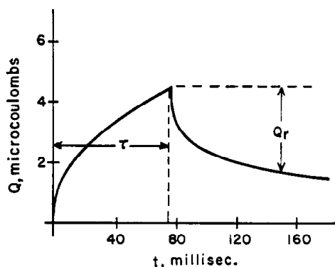
Figure 3. Charge-time curve for double potential-step chronocoulometry with 1mM Cd(NO 3 ) 2 in 1F NaNO 3
